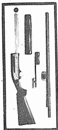
The Franchi 520 is made up of four main units. Stock and action. Barrel Breech bolt and cocking rod. Fore end. No tools are required.
