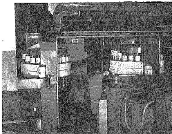
• The two Benzoni moulds in action.
